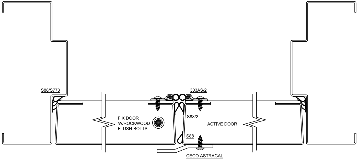
HEADER/JAMB VIEW VIEW OF FRAME AND DOOR PERIMETER
