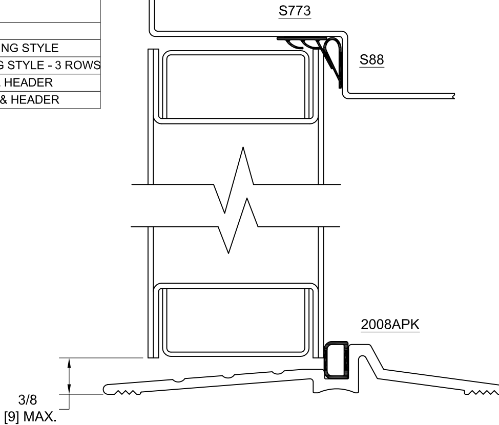
HEADER/JAMB VIEW VIEW OF FRAME AND DOOR PERIMETER
