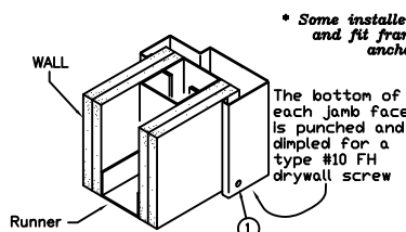
STANDARD SILL ANCHOR
