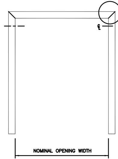
DOUBLE OPENING ELEVATION
