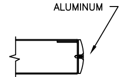
BULLNOSE 4783-1/4" ALUMINUM (screwed on) (1-3/4" thick double acting doors only)
