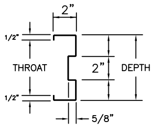
TYPE ②A PROFILE (Strike-Jamb)
