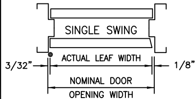
HORIZONTAL SECTION
