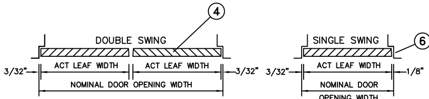
HORIZONTAL SECTIONS
