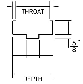
TYPICAL SECTION
