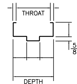
TYPICAL SECTION
