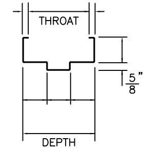
TYPICAL SECTION
