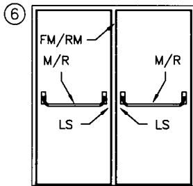
PAIR OF DOORS WITH HOLLOW METAL OR HARDWARE MULLION
