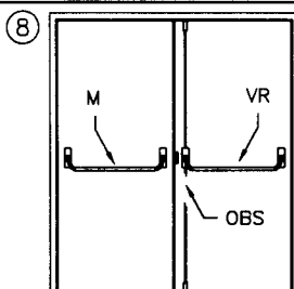
PAIR OF DOORS WITH OPEN BACK STRIKE
